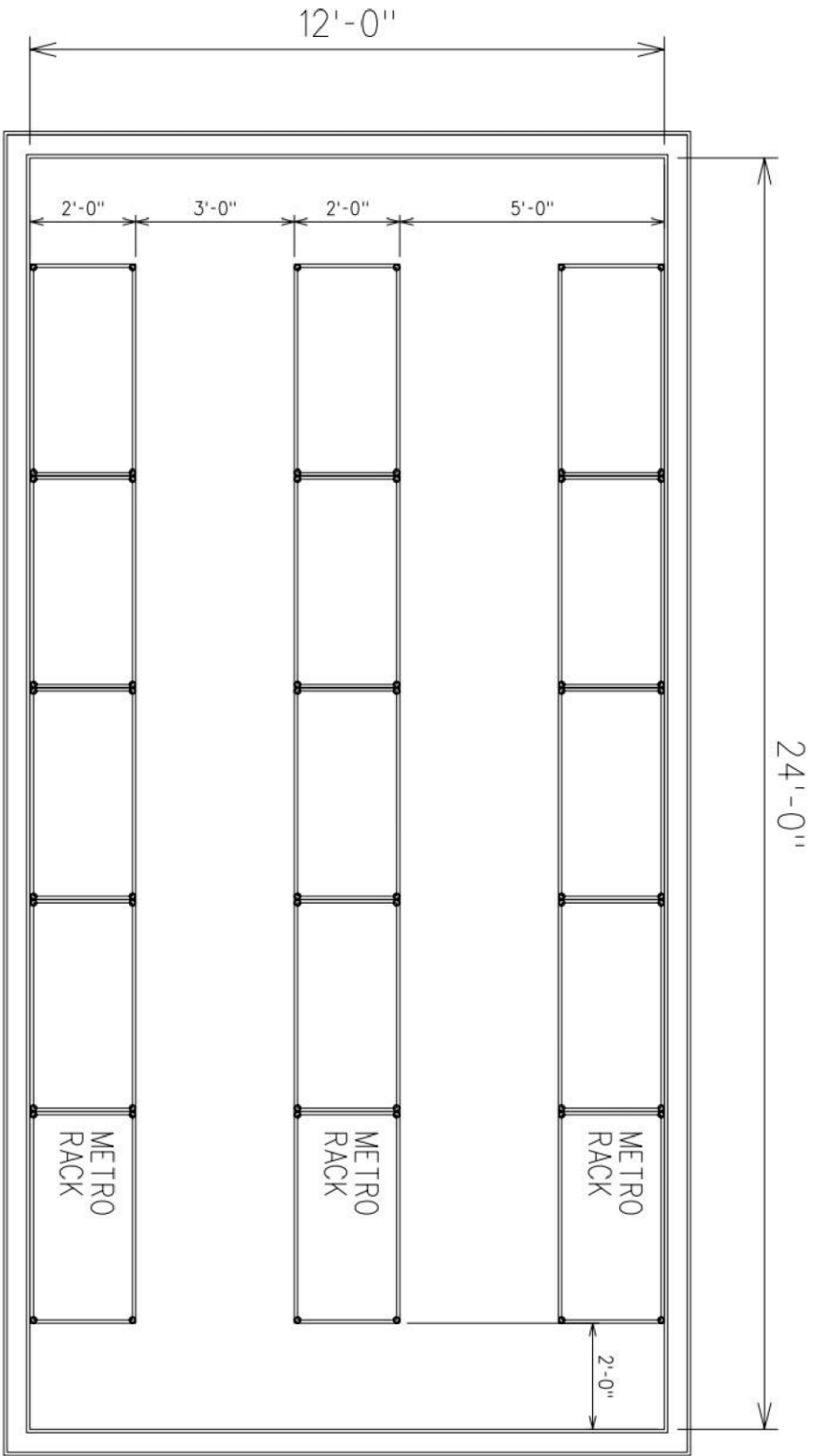
FRUITING ROOM LAYOUT - PLAN
